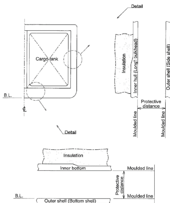
Fig. 2.5-2 Protective distance to semi-membrane tank
